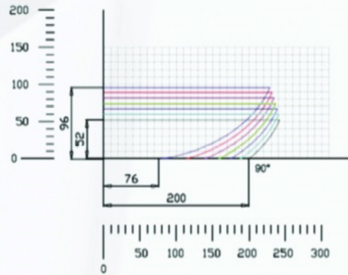
Cutting Graph at 45° tilted head
