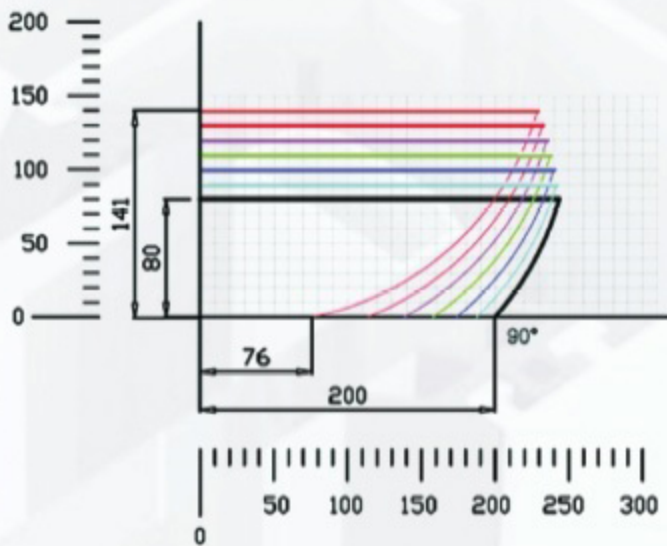
Cutting Graph at 90°
